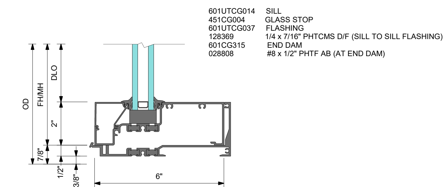
3 DETAIL 3 SILL
