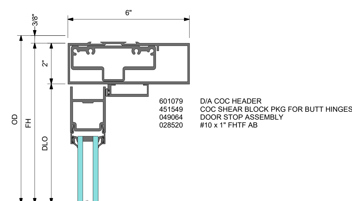
DOOR HEADER WITH LCN CONCEALED CLOSER AND BUTT HINGES
