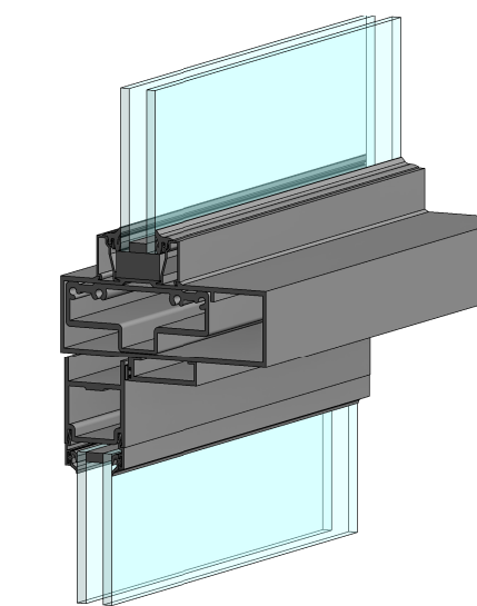
3D-VIEW
