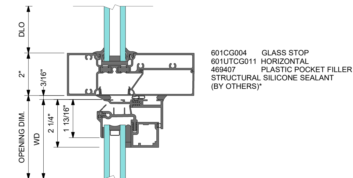
1 VENT HEAD
