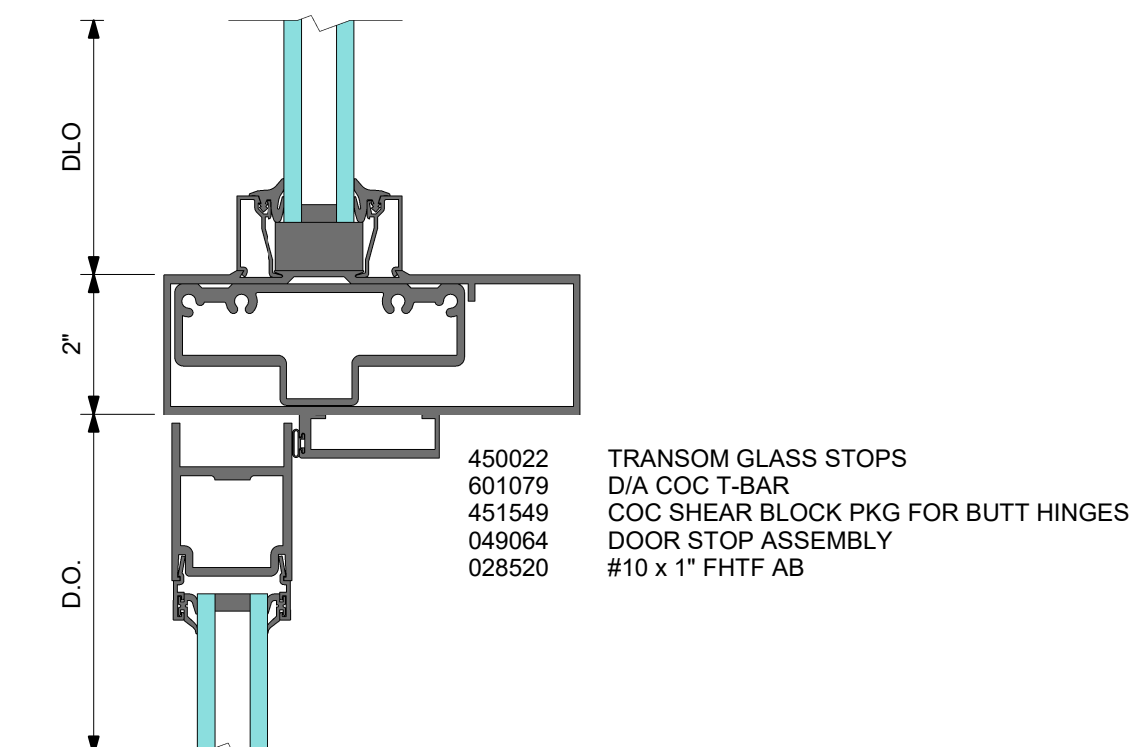
DOOR TRANSOM BAR WITH LCN CONCEALED CLOSER AND BUTT HINGES
