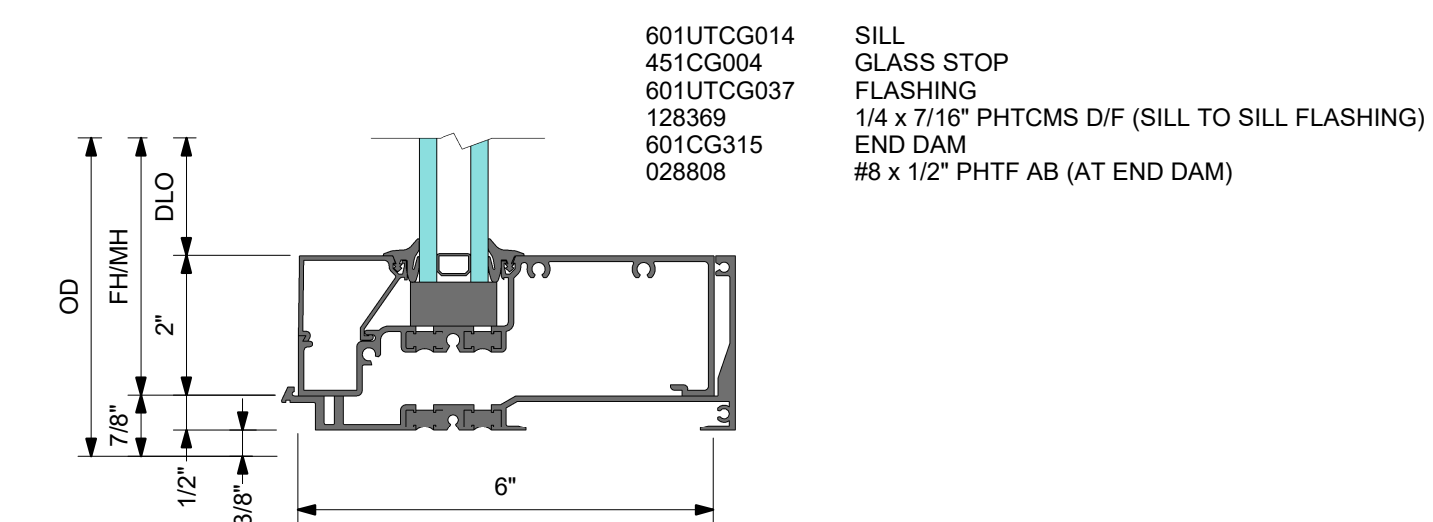
3 DETAIL 3 SILL
