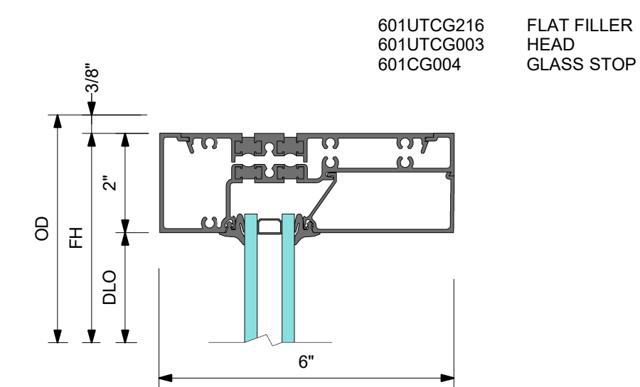
1 DETAIL 1 HEAD
