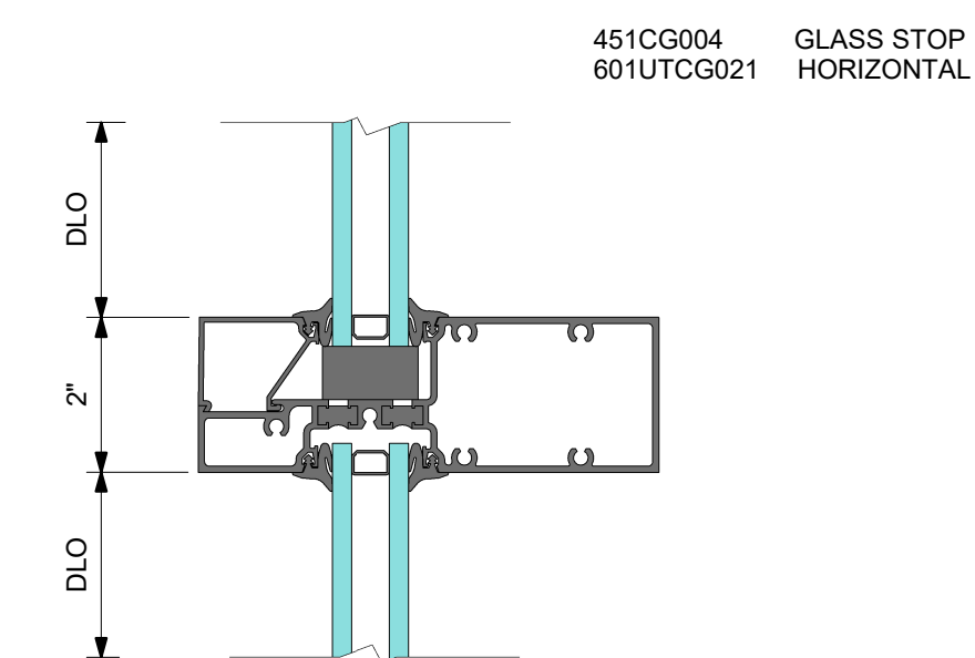
2 DETAIL 2 HORIZONTAL
