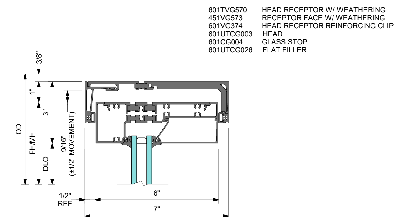
1 DETAIL 1 HEAD WITH HD RECEPTOR
