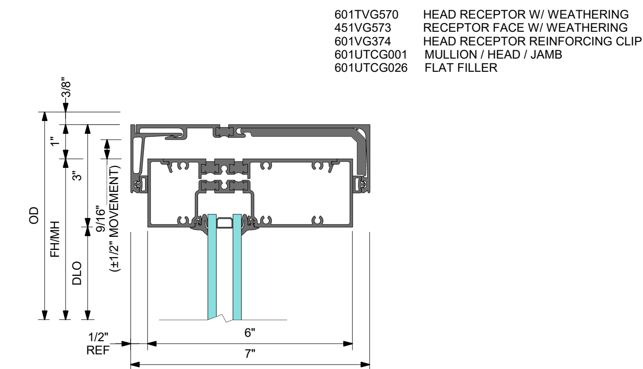
1 DETAIL 1 HEAD WITH HD RECEPTOR
