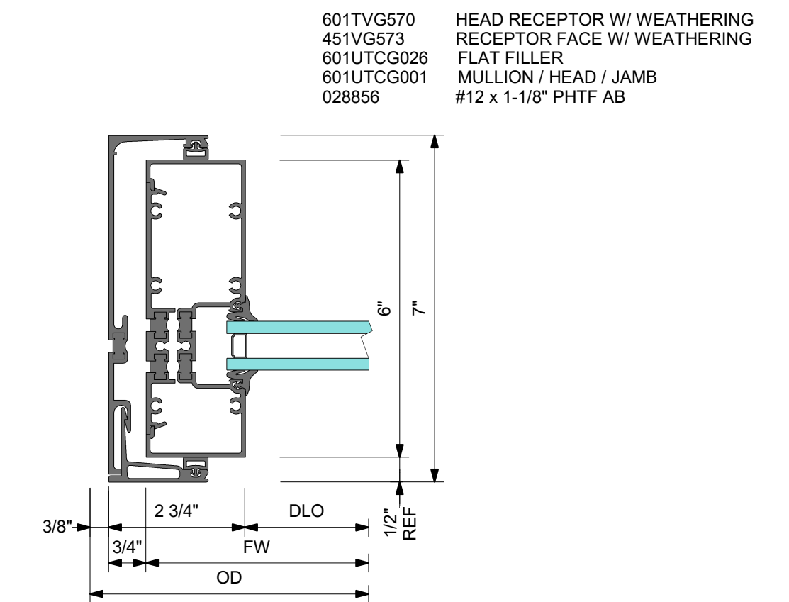
4 DETAIL 4 JAMB WITH HD RECEPTOR
