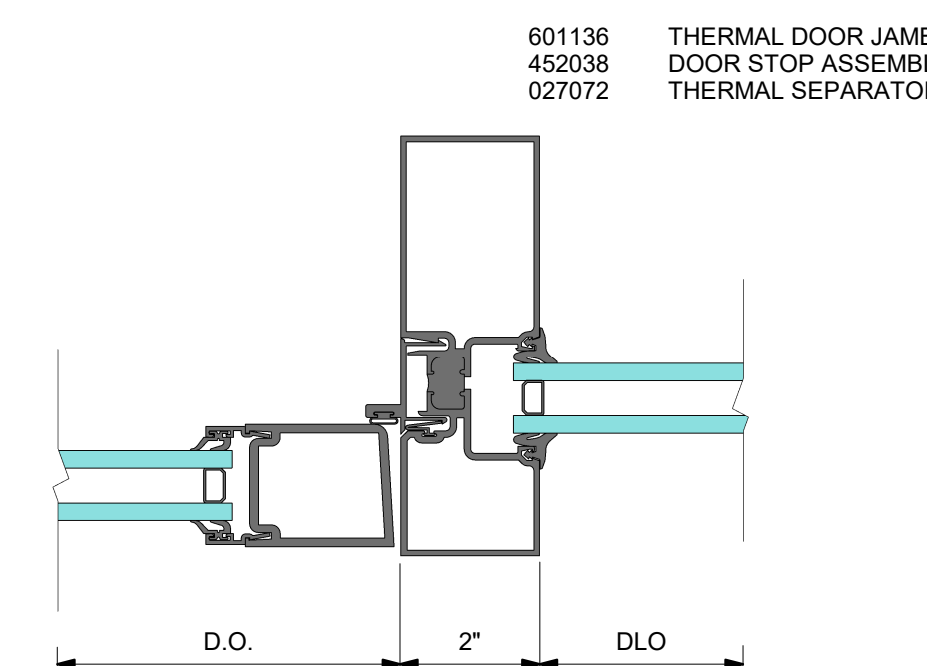
5 DETAIL 5 DOOR JAMB WITH SIDELITE
