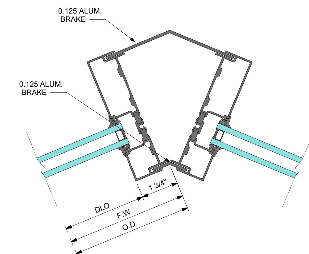
601UTCG010 FEMALE EXPANSION MULLION HALF
