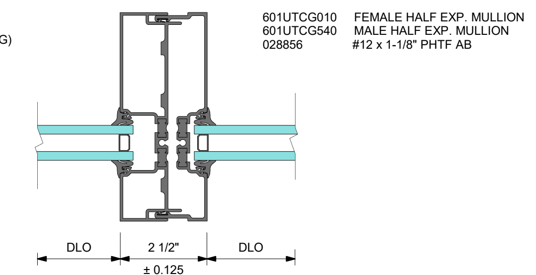
6 DETAIL 6 EXPANSION MULLION
