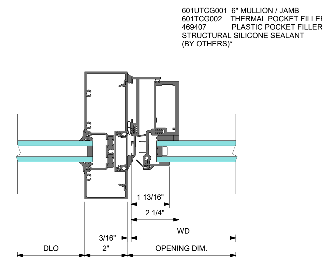
3 VENT @ RIGHT
