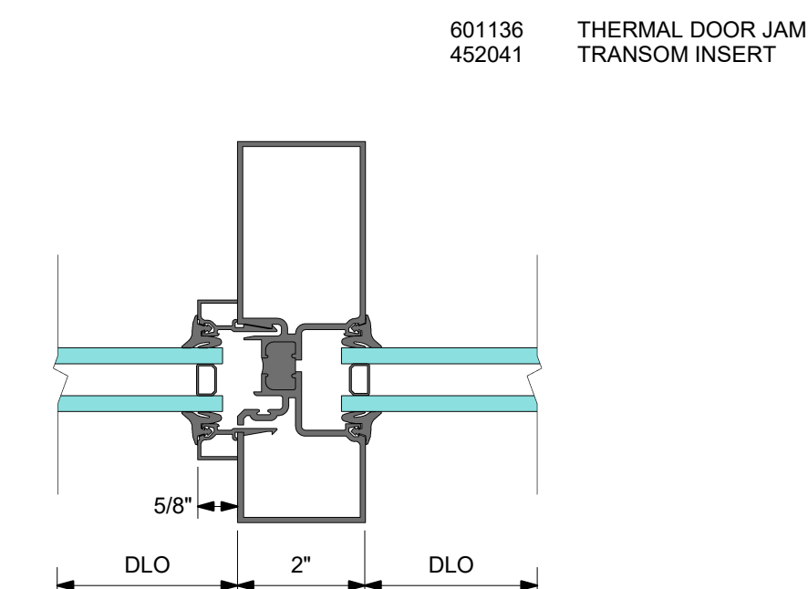
5A DETAIL 5A TRANSOM JAMB WITH SIDELITE
