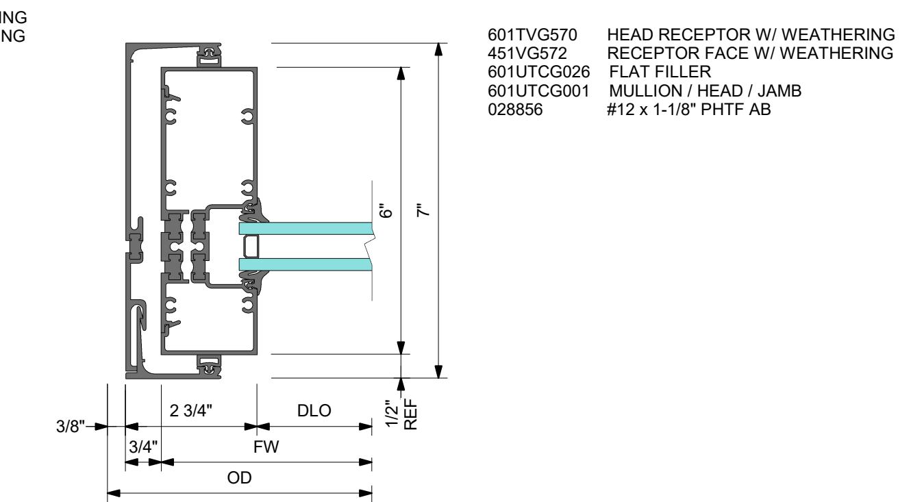
4 DETAIL 4 JAMB WITH RECEPTOR
