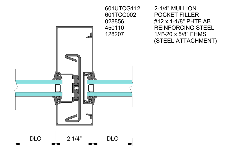
5 DETAIL 5 - 2-1/4" VERTICAL MULLION WITH STEEL
