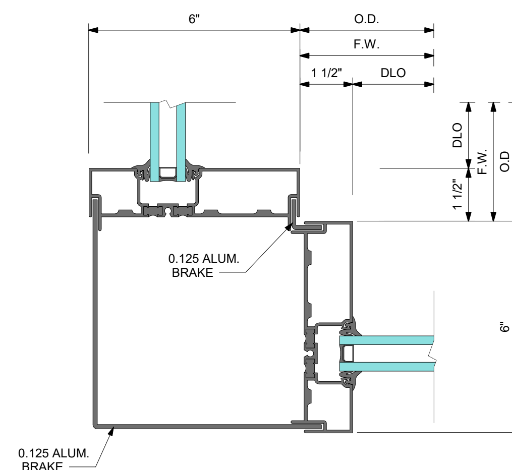
90° OUTSIDE CORNER WITH BRAKE METAL
