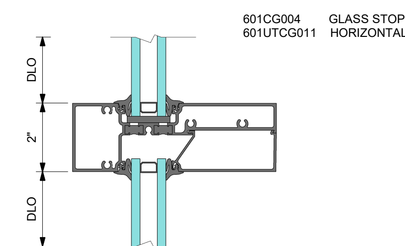
2 DETAIL 2 HORIZONTAL
