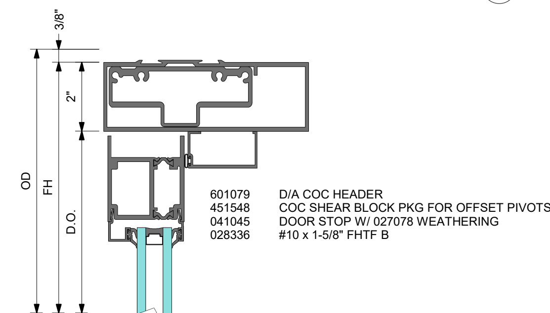
DOOR HEADER WITH KAWNEER CONCEALED CLOSER AND OFFSET PIVOTS
