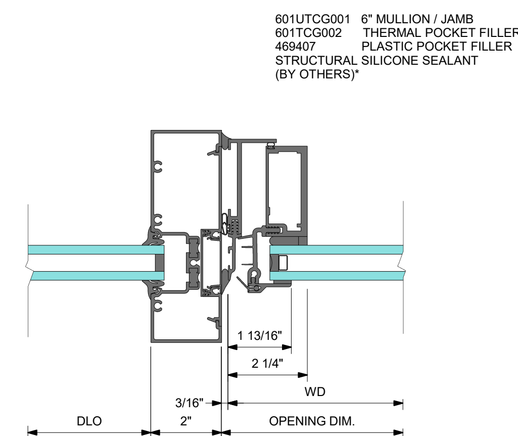
3 VENT @ RIGHT
