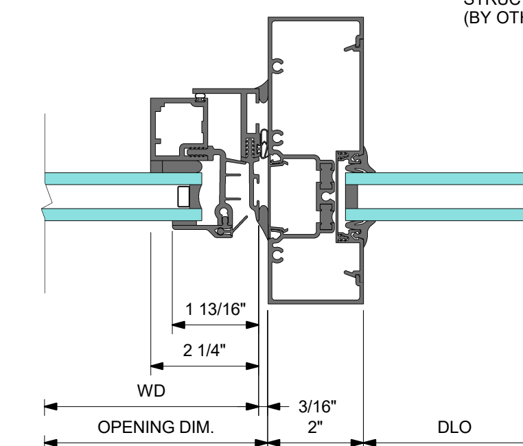
4 VENT @ LEFT
