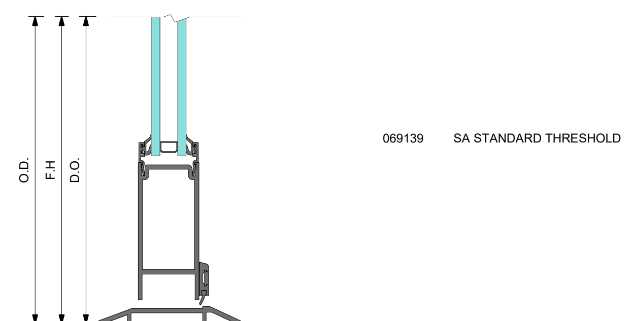
3 DETAIL 3 THRESHOLD
