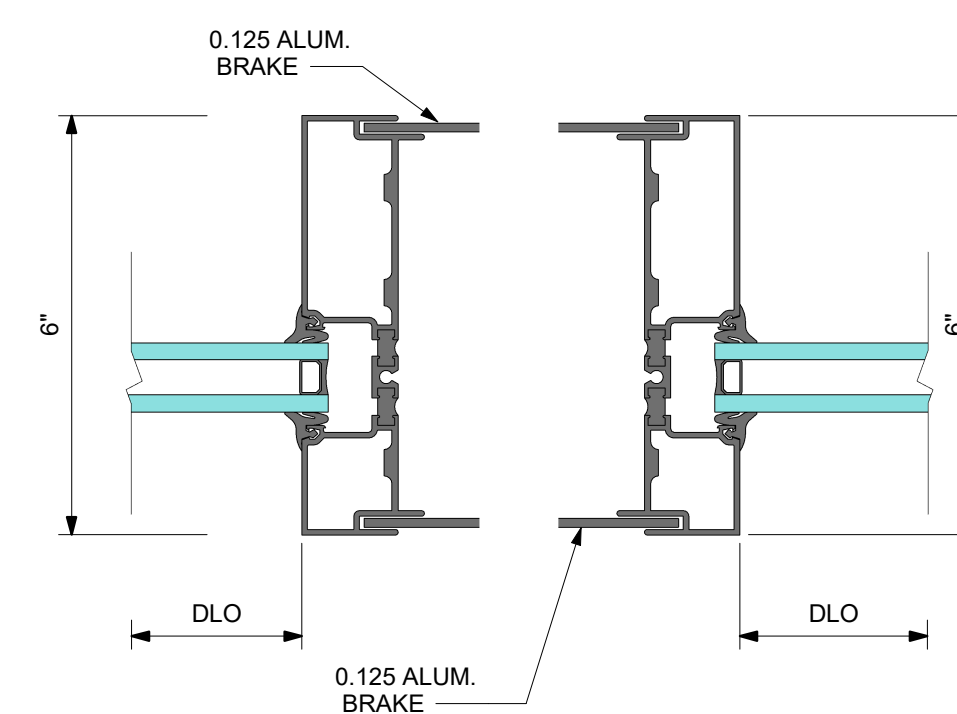
601UTCG010 FEMALE EXPANSION MULLION HALF
