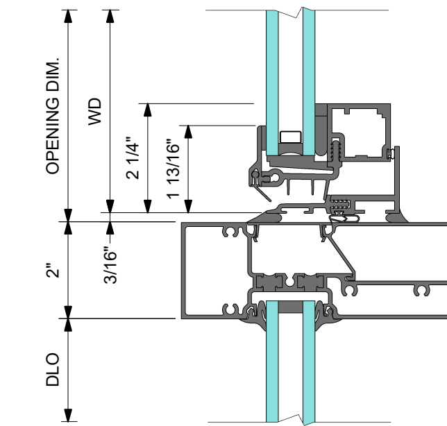
2 VENT SILL
