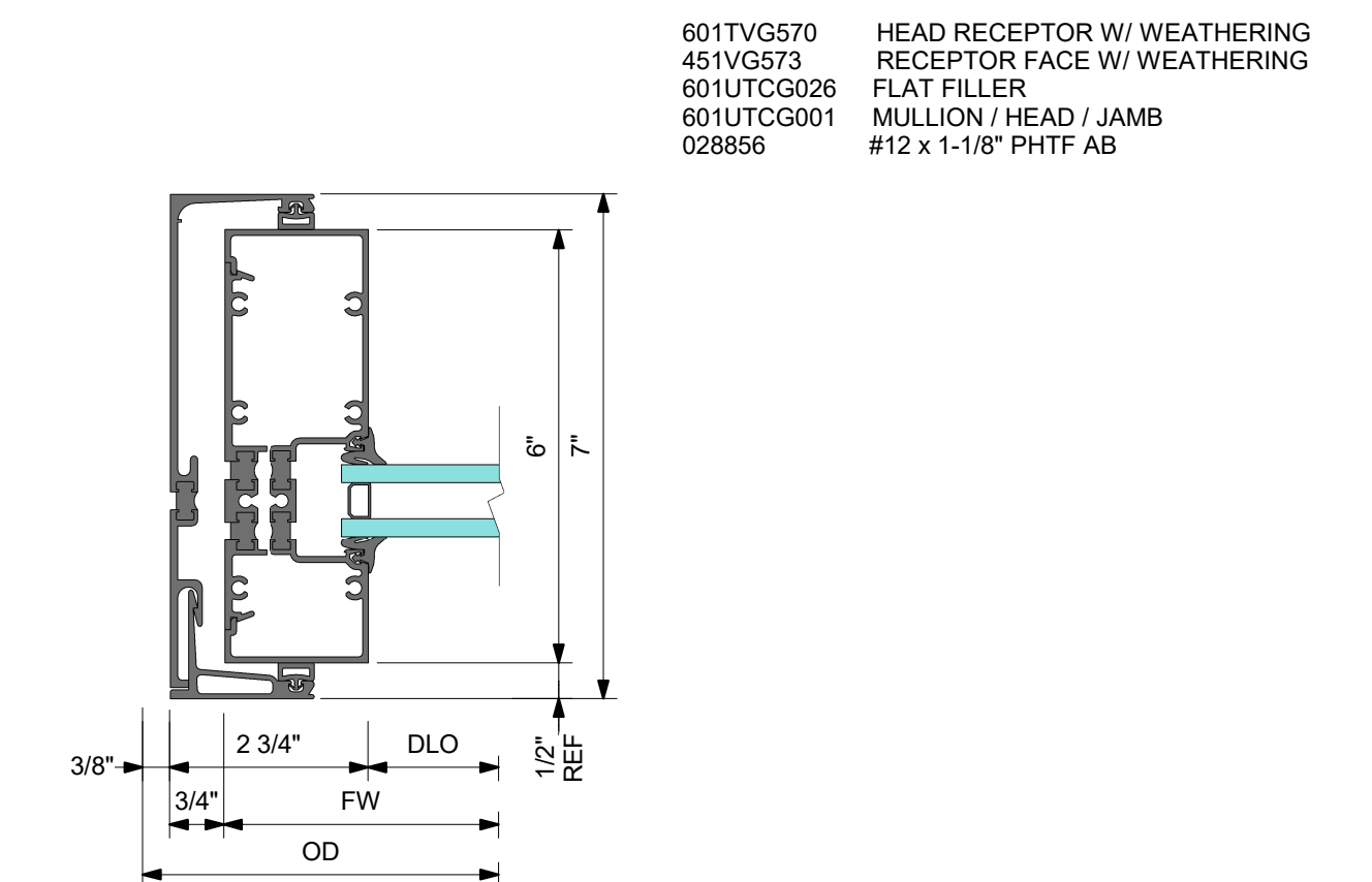
4 DETAIL 4 JAMB WITH HD RECEPTOR
