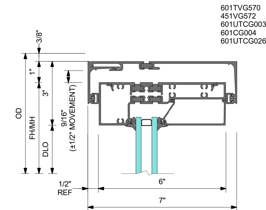
1 DETAIL 1 HEAD WITH RECEPTOR
