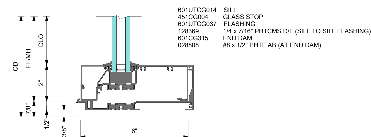
3 DETAIL 3 SILL
