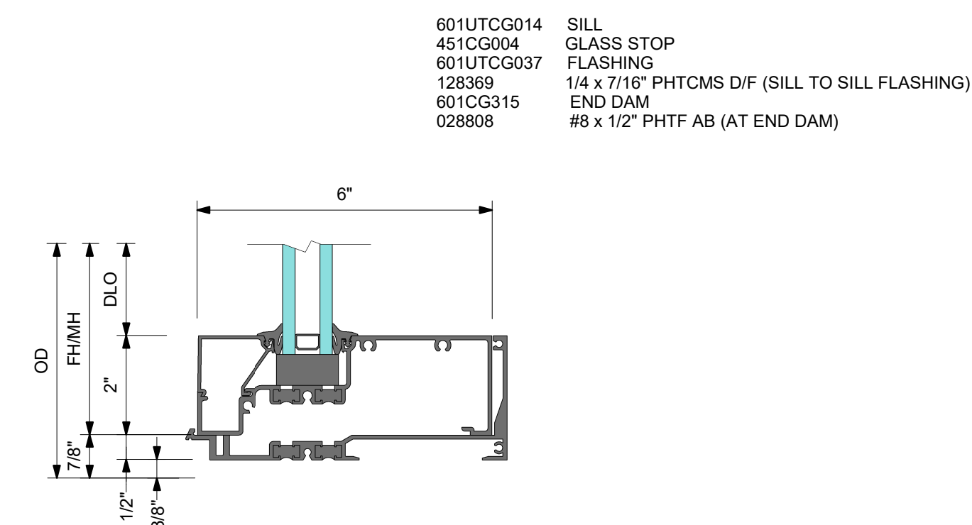
3 DETAIL 3 SILL
