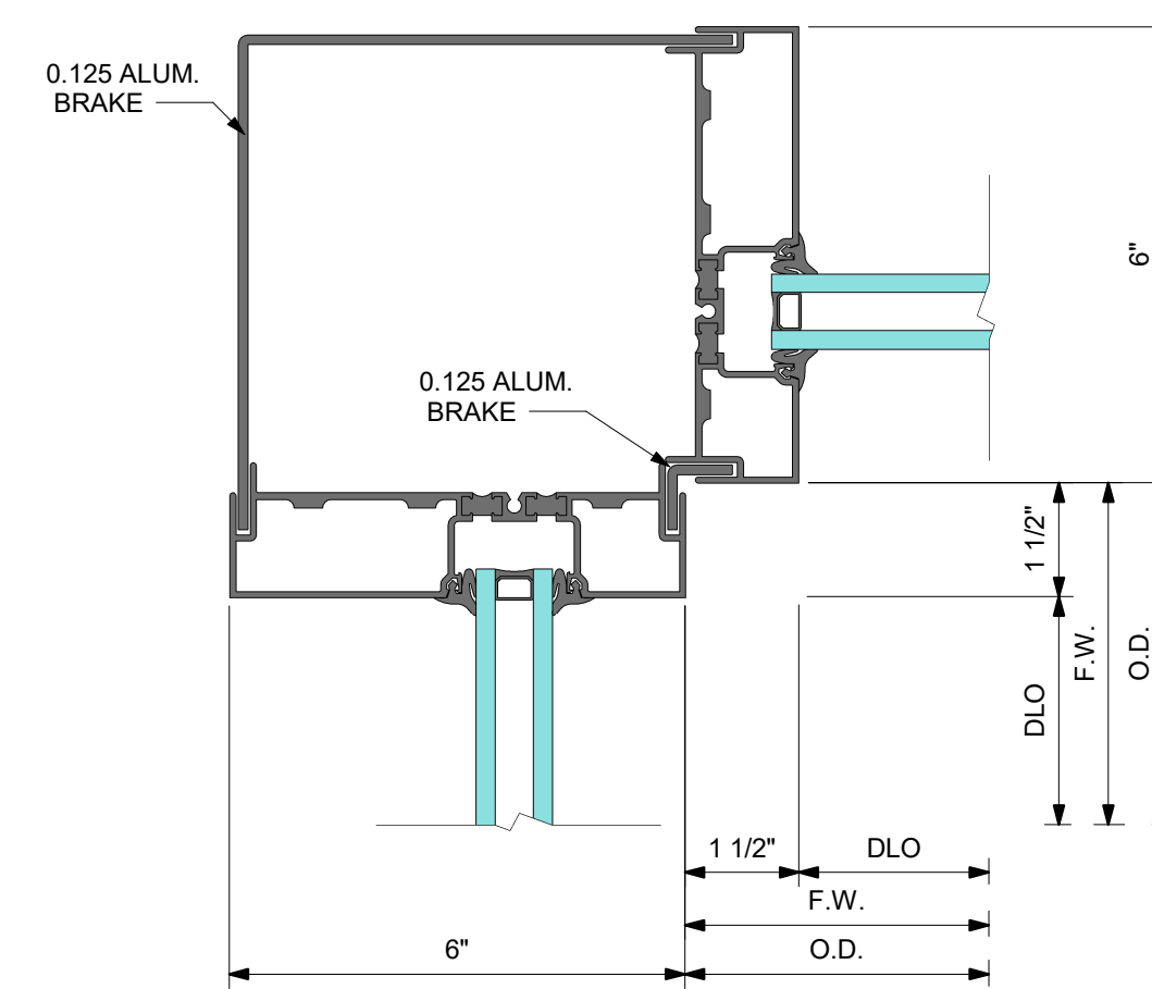
90° INSIDE CORNER WITH BRAKE METAL
