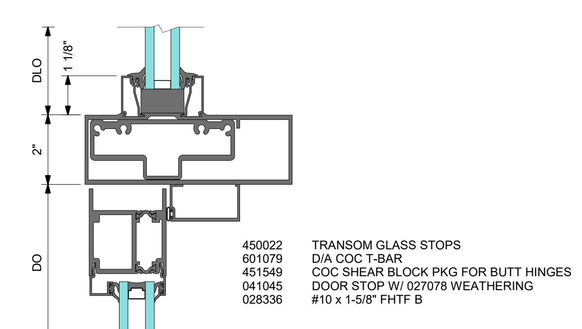
DOOR TRANSOM BAR WITH KAWNEER CONCEALED CLOSER AND BUTT HINGES
