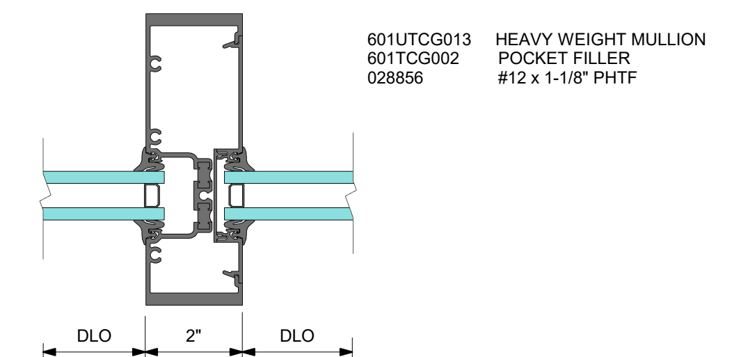
5 DETAIL 5 HEAVY WEIGHT VERTICAL MULLION
