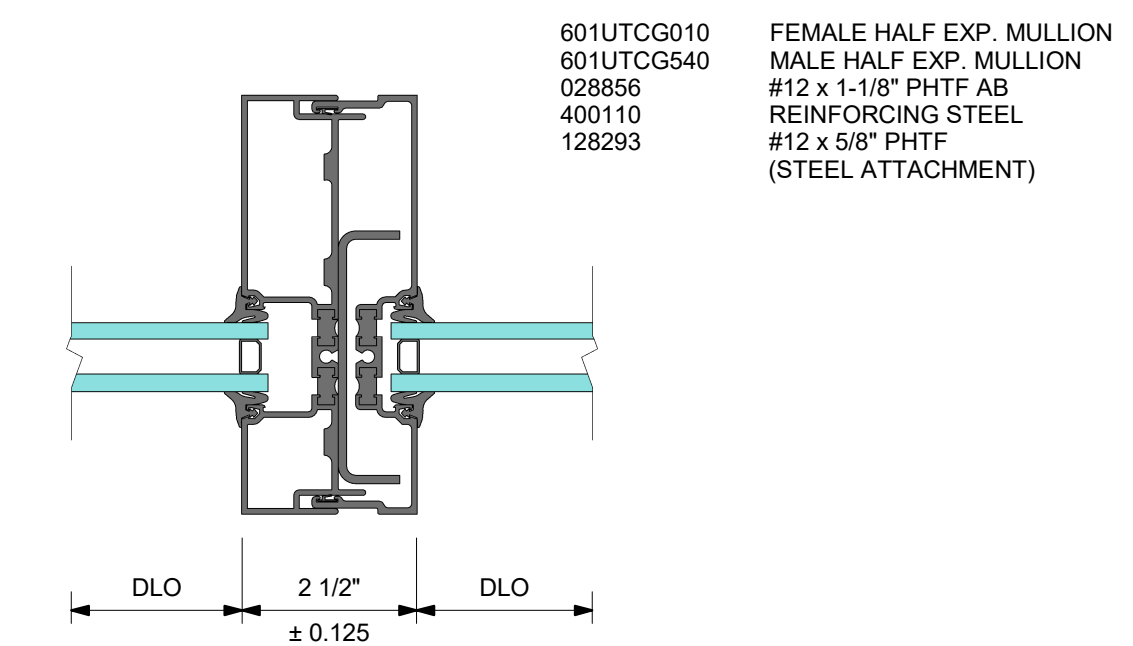
5 DETAIL 5 EXPANSION MULLION WITH STEEL
