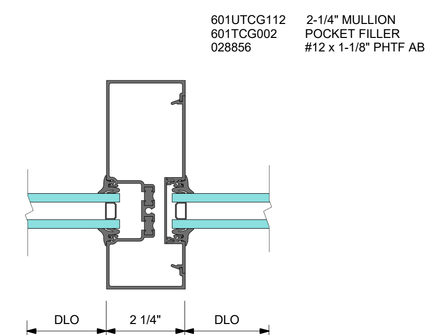
6 DETAIL 6 - 2-1/4" VERTICAL MULLION
