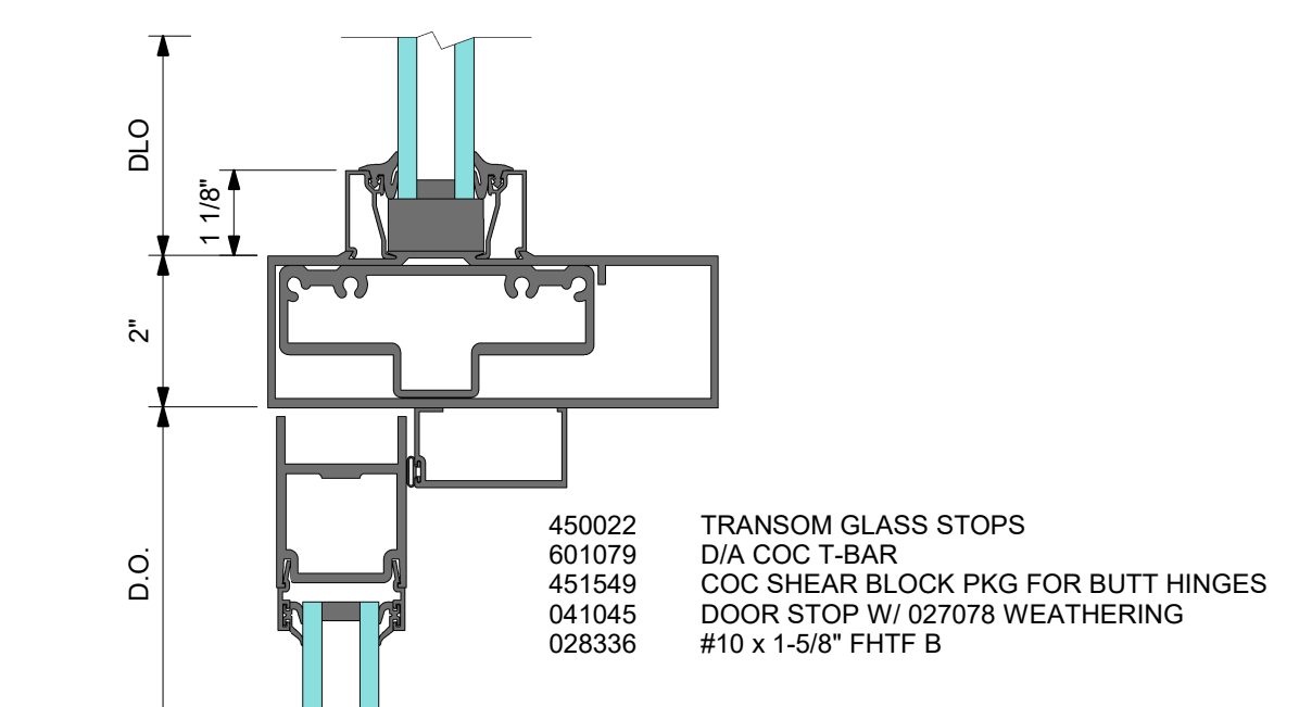
DOOR TRANSOM BAR WITH KAWNEER CONCEALED CLOSER AND BUTT HINGES
