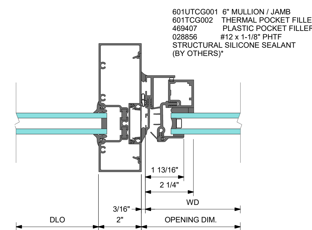
3 VENT @ RIGHT
