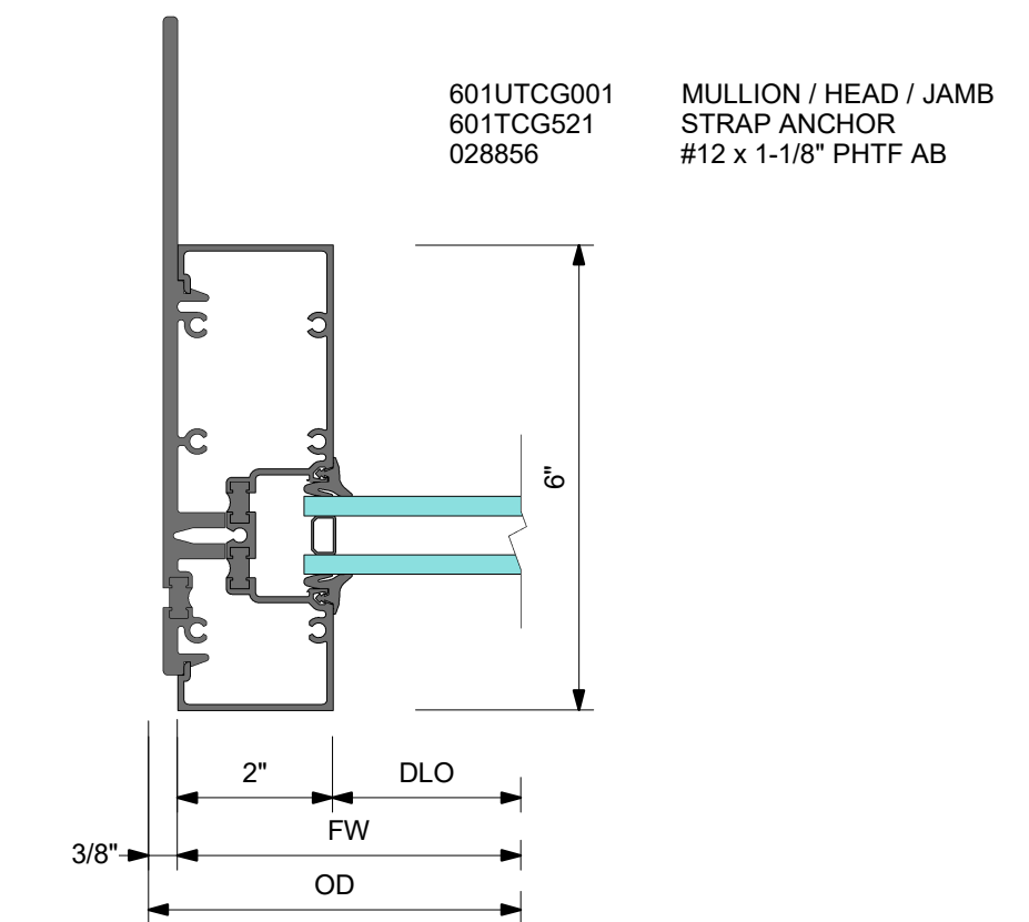
4 DETAIL 4 JAMB WITH STRAP ANCHOR
