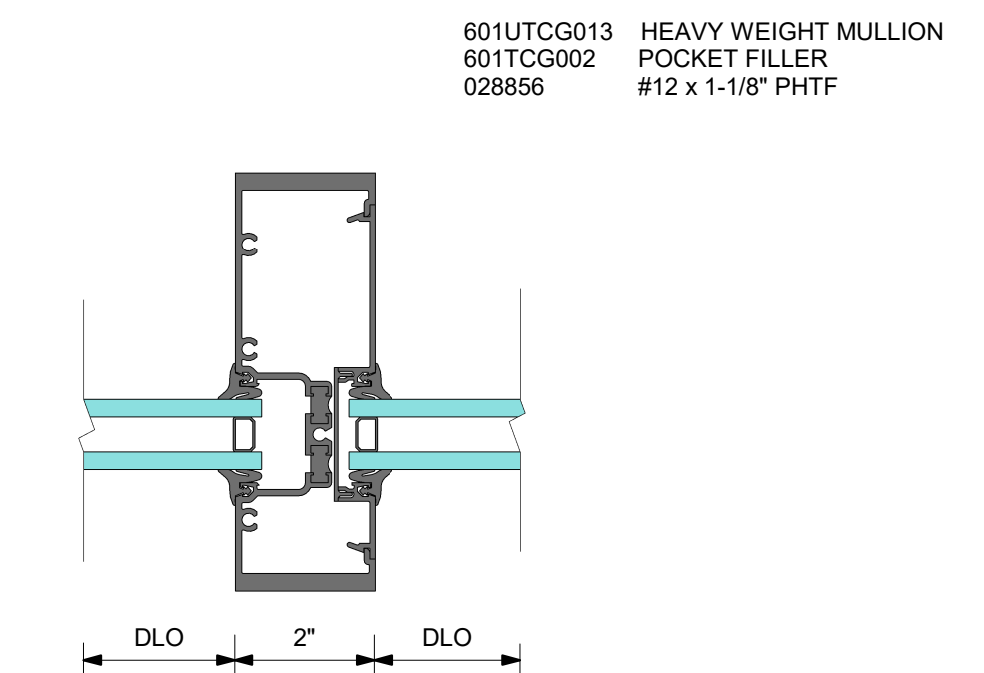
5 DETAIL 5 HEAVY WEIGHT VERTICAL MULLION
