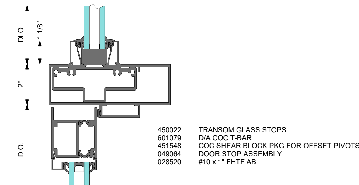
DOOR TRANSOM BAR WITH LCN CONCEALED CLOSER AND OFFSET PIVOTS
