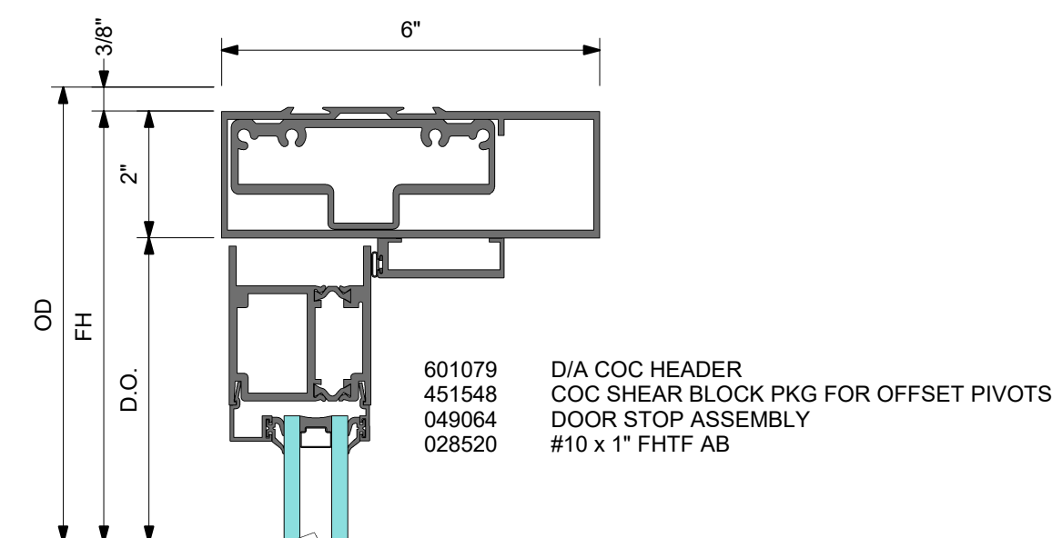
DOOR HEADER WITH LCN CONCEALED CLOSER AND OFFSET PIVOTS
