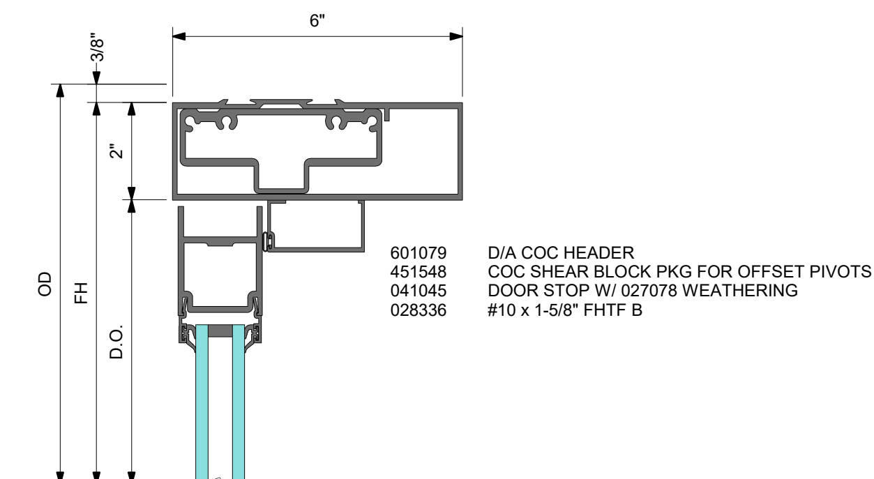
DOOR HEADER WITH KAWNEER CONCEALED CLOSER AND OFFSET PIVOTS
