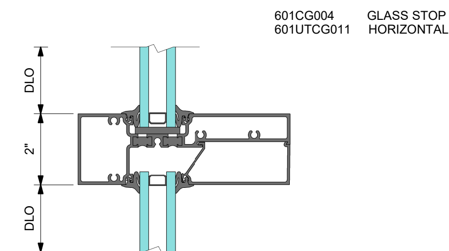
2 DETAIL 2 HORIZONTAL
