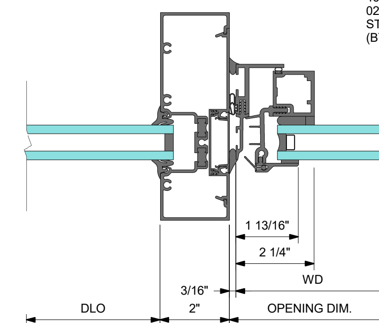
3 VENT @ RIGHT
