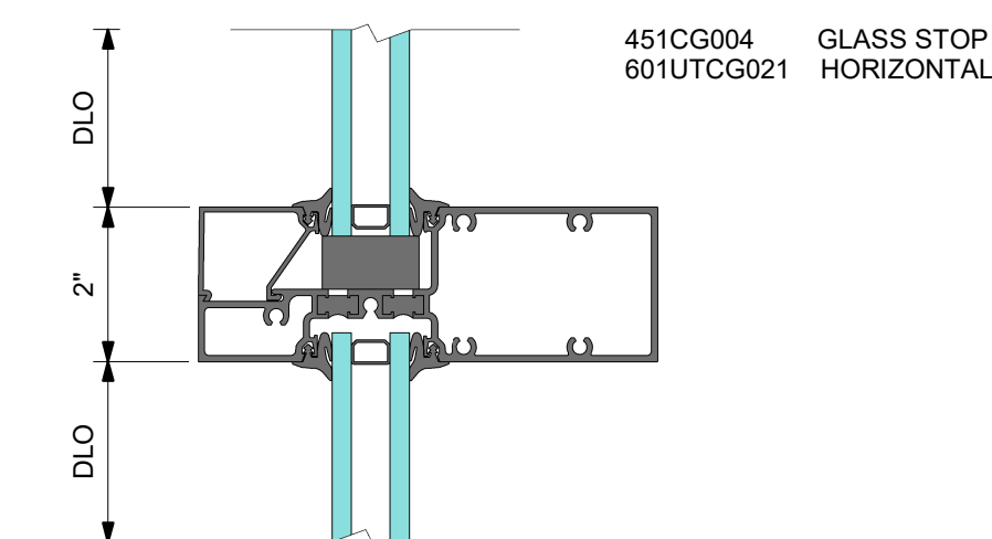
2 DETAIL 2 HORIZONTAL
