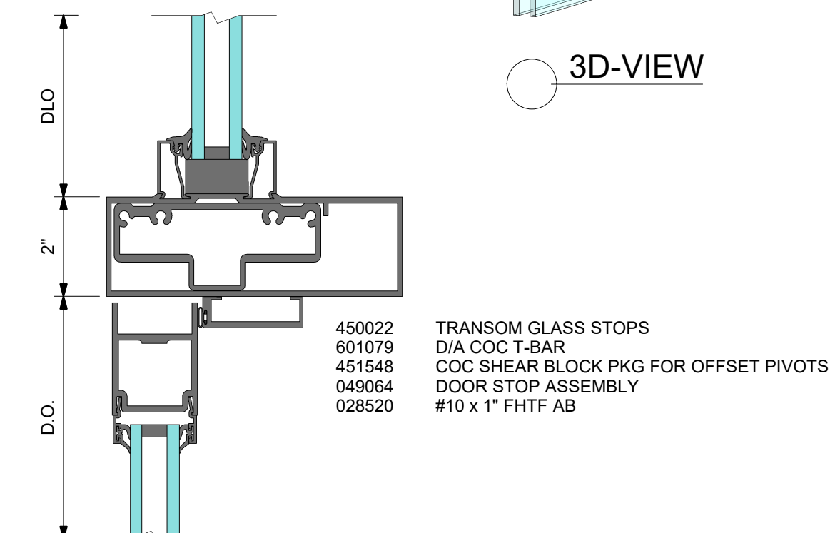
DOOR TRANSOM BAR WITH LCN CONCEALED CLOSER AND OFFSET PIVOTS
