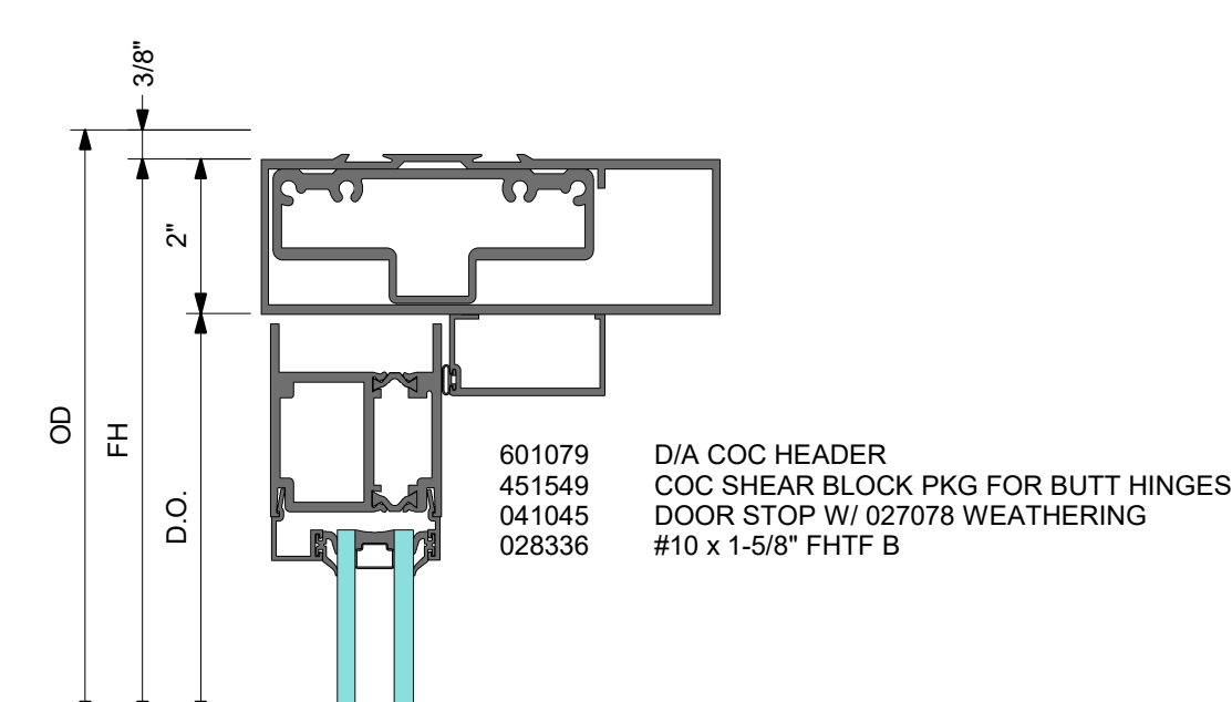
DOOR HEADER WITH KAWNEER CONCEALED CLOSER AND BUTT HINGES
