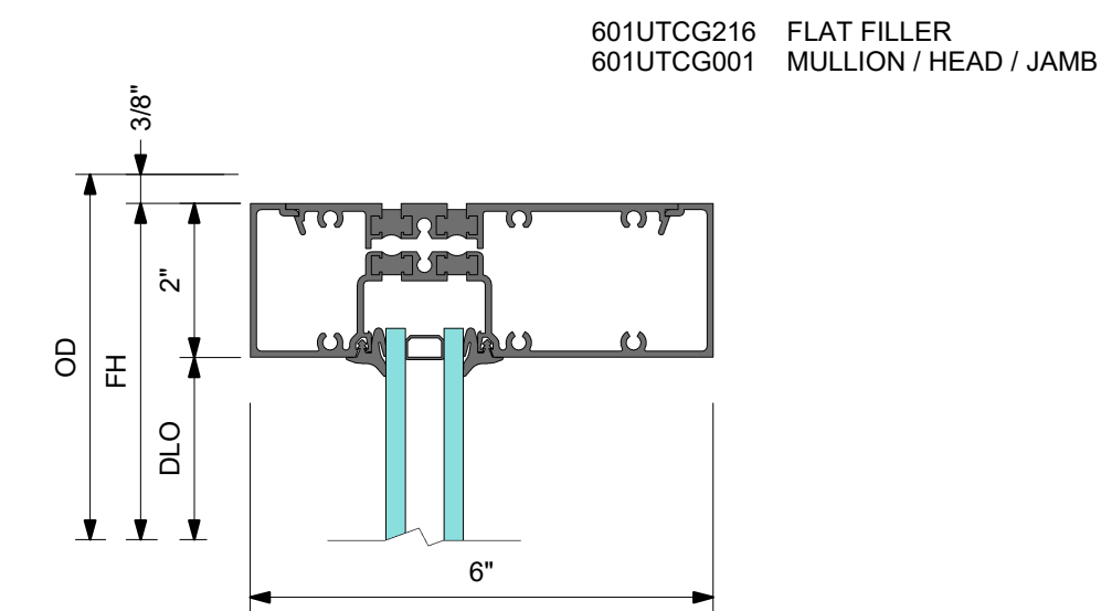
1 DETAIL 1 HEAD
