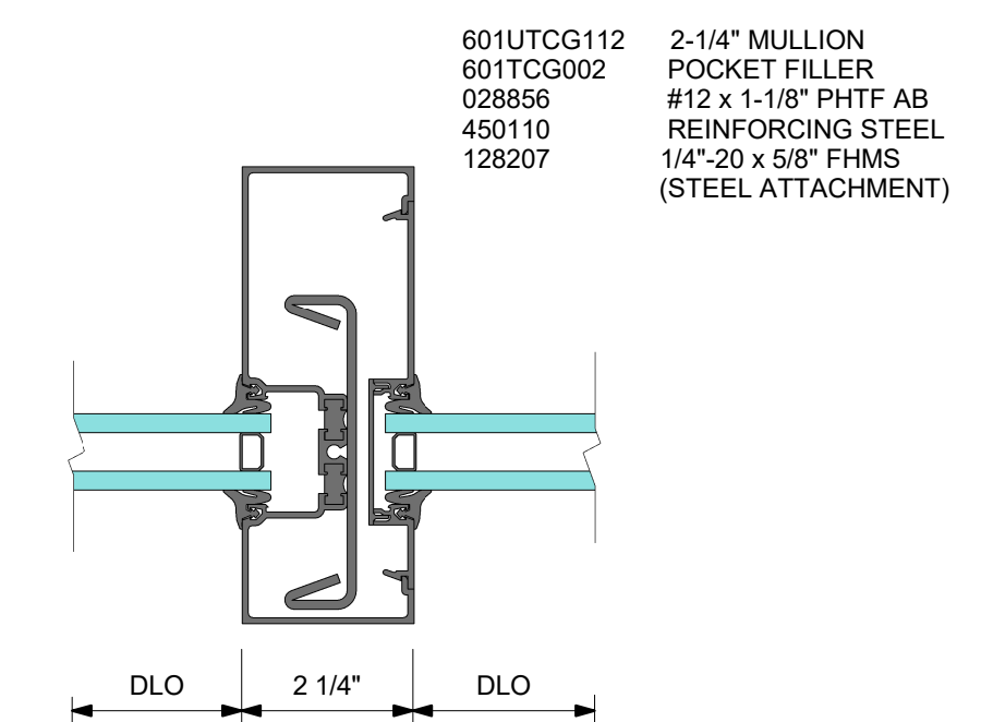
5 DETAIL 5 - 2-1/4" VERTICAL MULLION WITH STEEL
