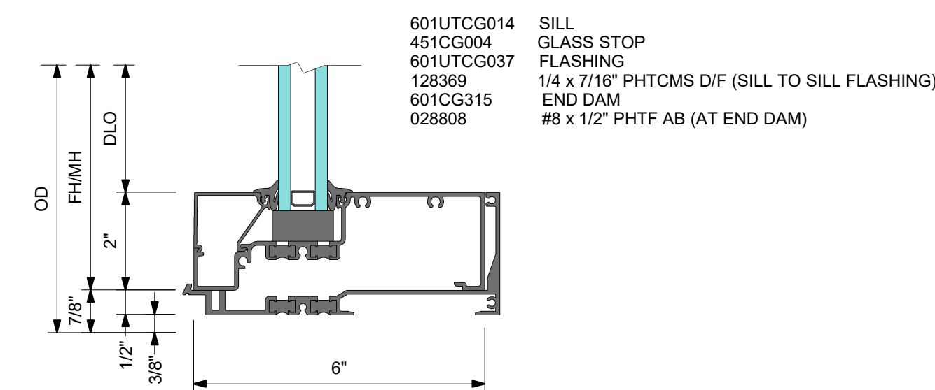
3 DETAIL 3 SILL
