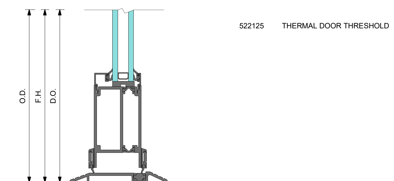
3 DETAIL 3 THRESHOLD
