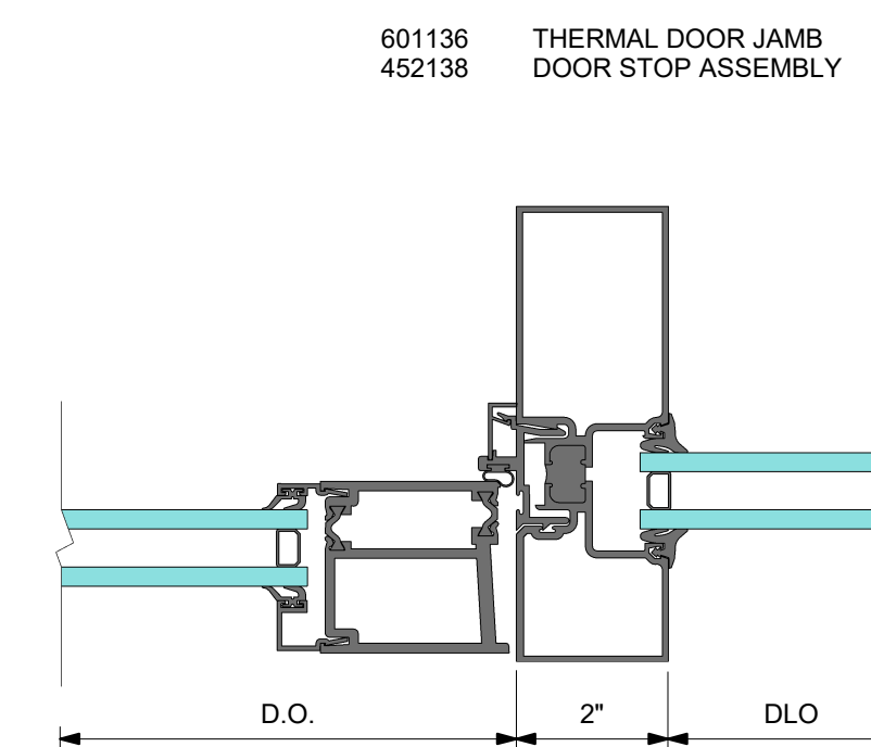
5 DETAIL 5 DOOR JAMB WITH SIDELITE
