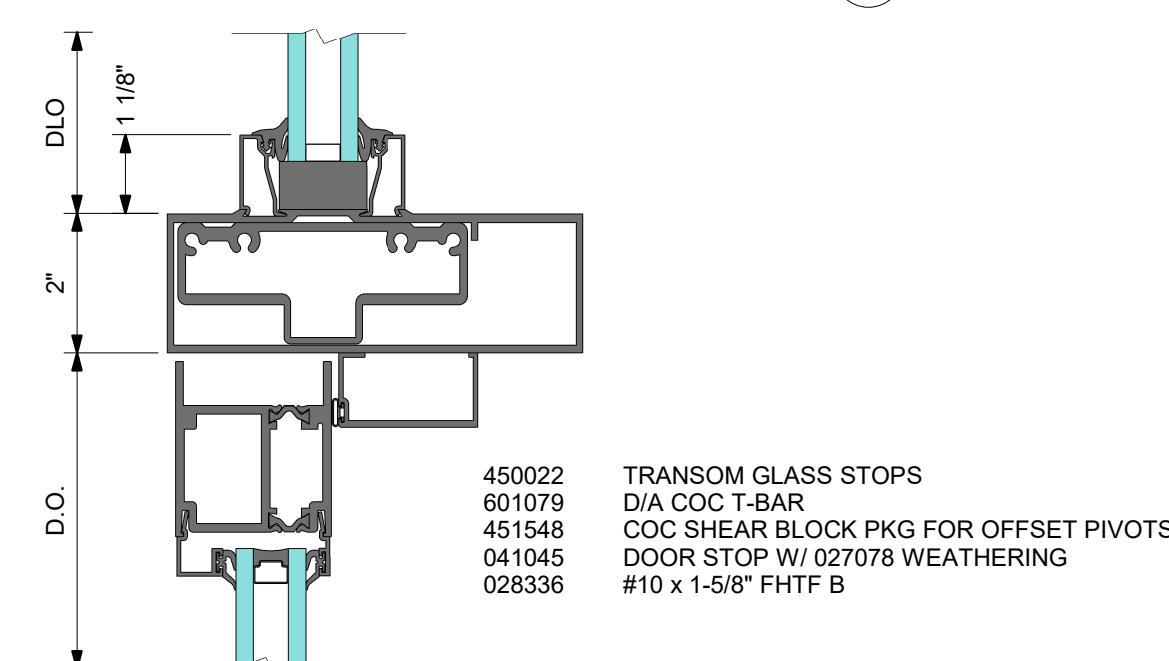
DOOR TRANSOM BAR WITH KAWNEER CONCEALED CLOSER AND OFFSET PIVOTS
