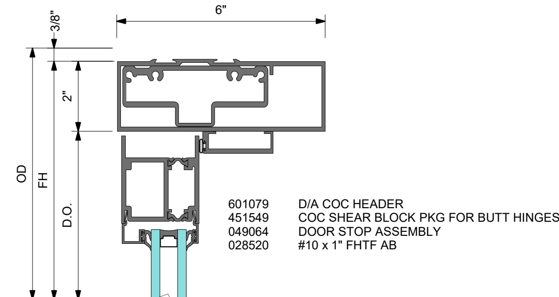
DOOR HEADER WITH LCN CONCEALED CLOSER AND BUTT HINGES
