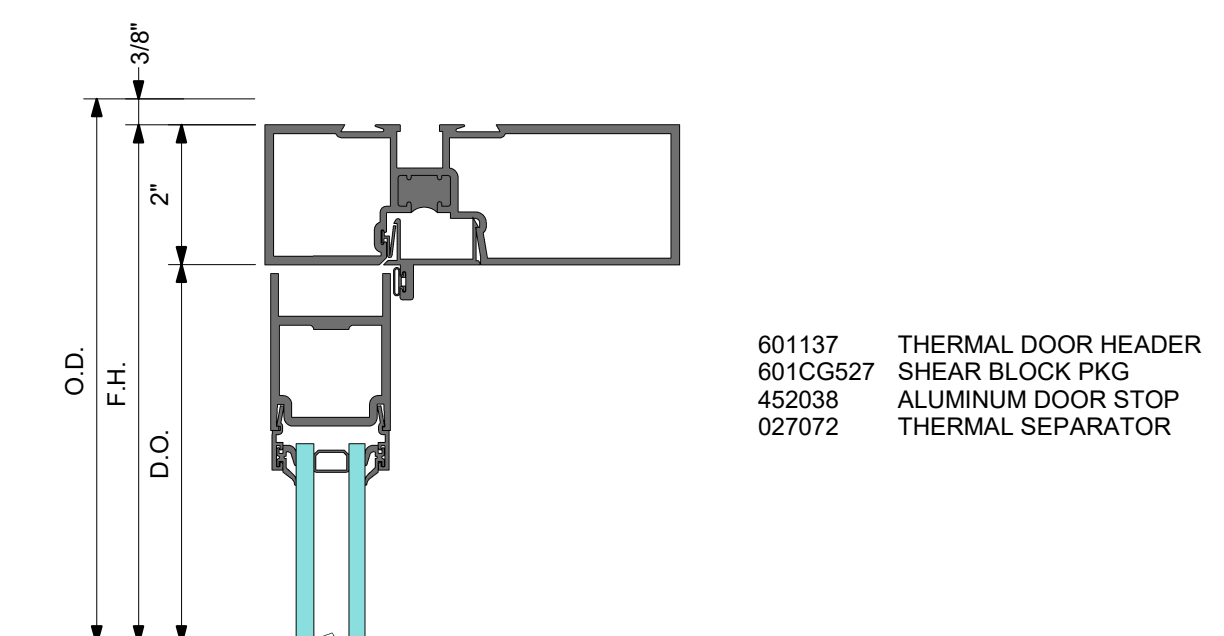
2A DETAIL 2A DOOR HEADER WITH SURFACE CLOSER
