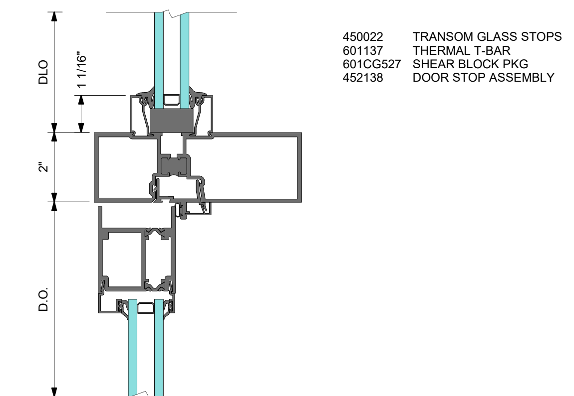
2 DETAIL 2 TRANSOM BAR WITH SURFACE CLOSER
