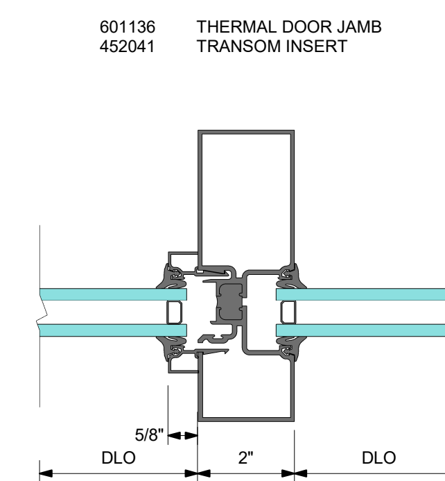
5A DETAIL 5A TRANSOM JAMB WITH SIDELITE
