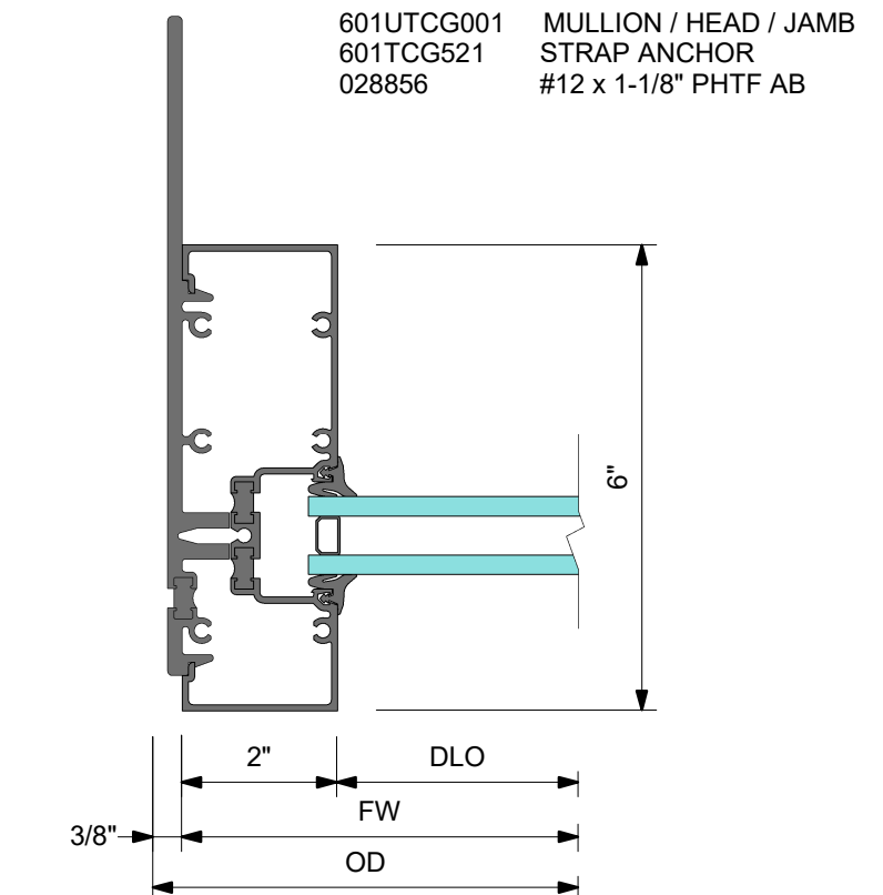
4 DETAIL 4 JAMB WITH STRAP ANCHOR
