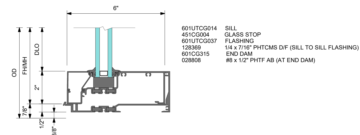
3 DETAIL 3 SILL
