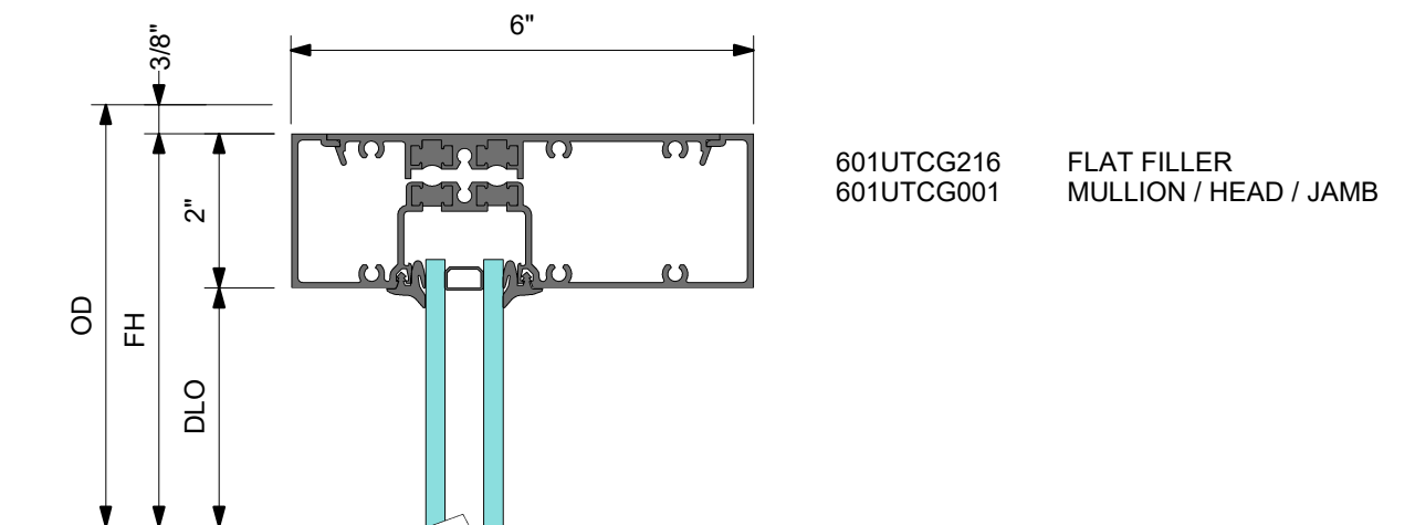
1 DETAIL 1 TRANSOM HEAD
