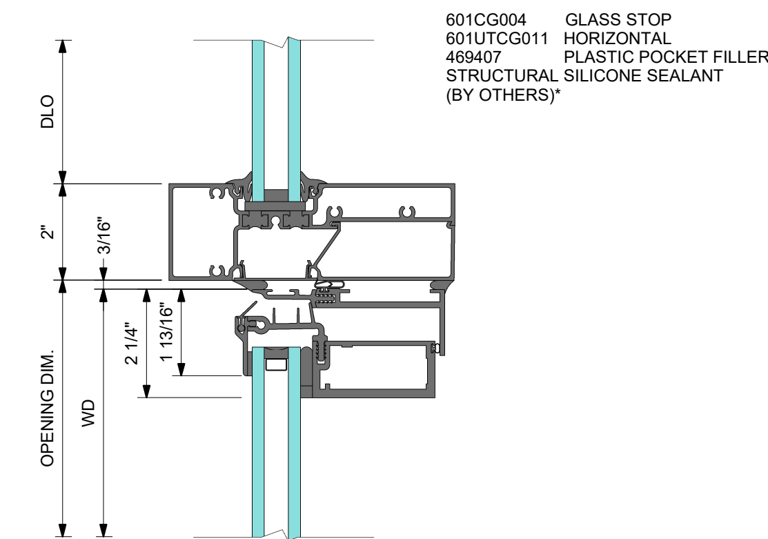
1 VENT HEAD
