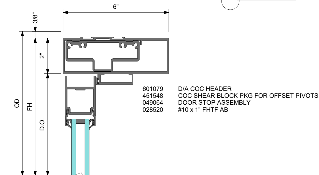
DOOR HEADER WITH LCN CONCEALED CLOSER AND OFFSET PIVOTS
