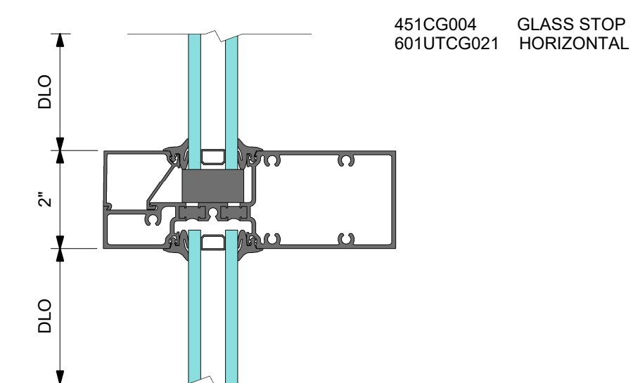
2 DETAIL 2 HORIZONTAL
