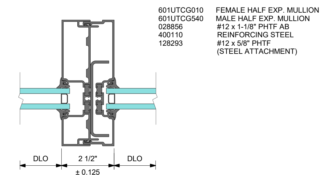
5 DETAIL 5 EXPANSION MULLION WITH STEEL
