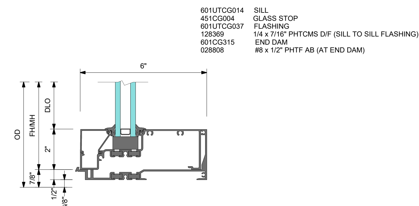
3 DETAIL 3 SILL
