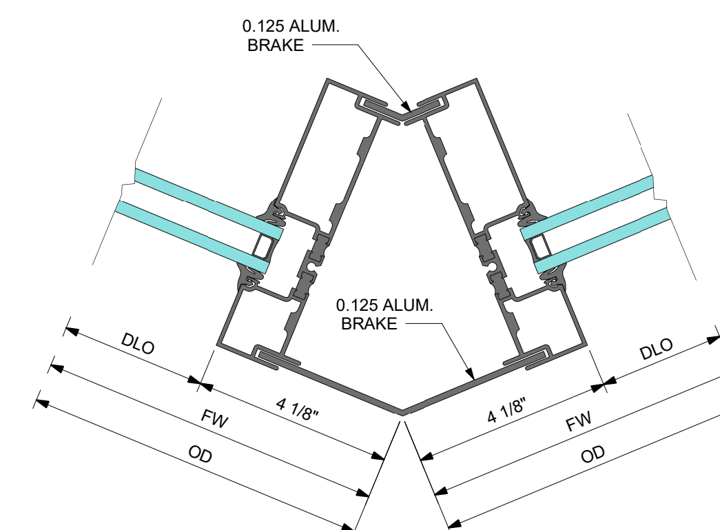
135° OUTSIDE CORNER WITH BRAKE METAL
