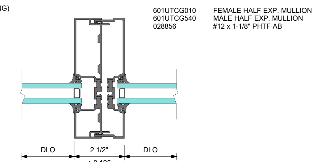
6 DETAIL 6 EXPANSION MULLION
