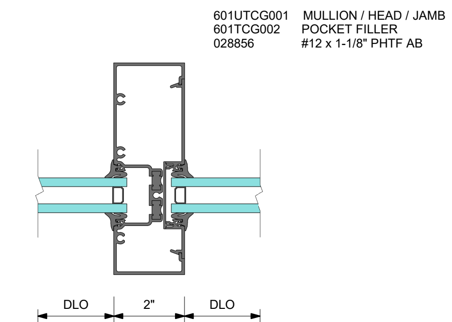
5 DETAIL 5 VERTICAL MULLION
