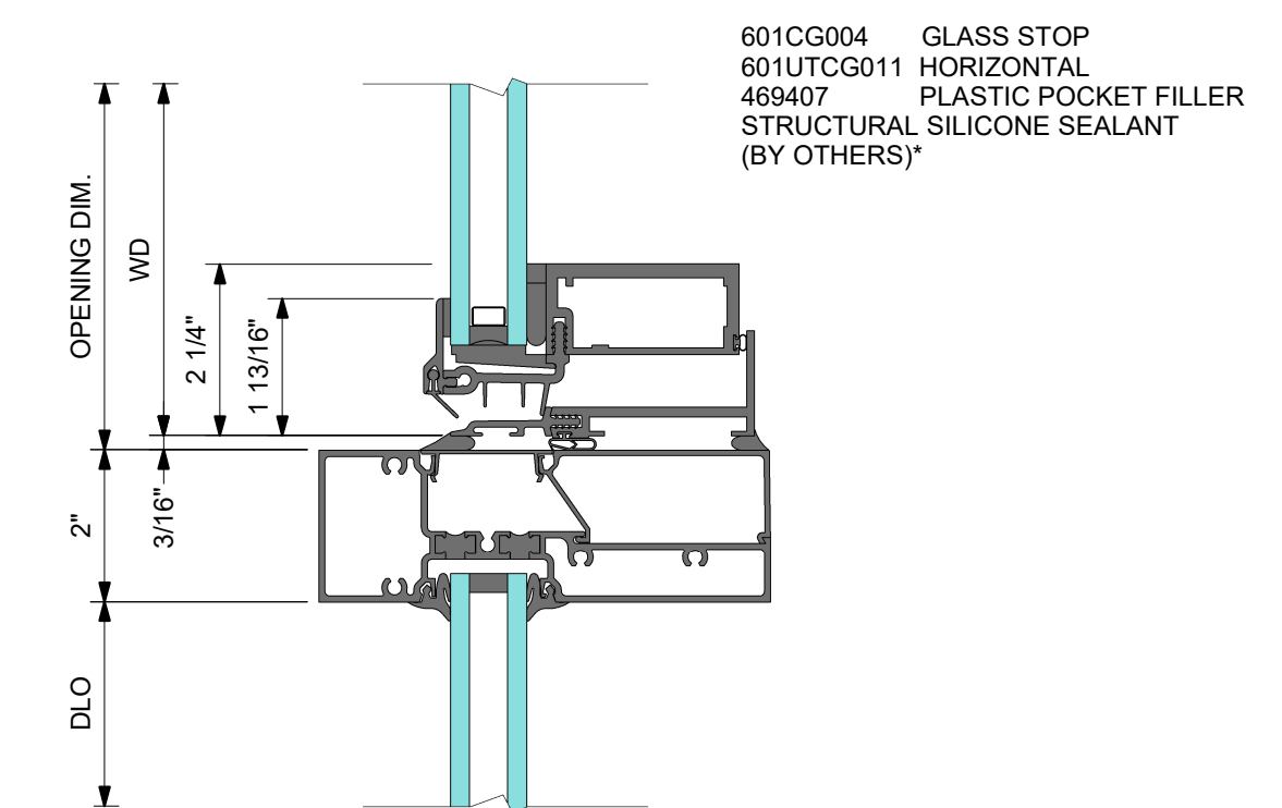
2 VENT SILL
