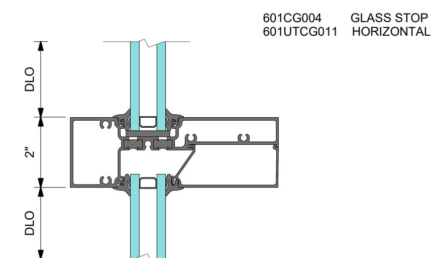
1 DETAIL 1 HEAD WITH STRAP ANCHOR
