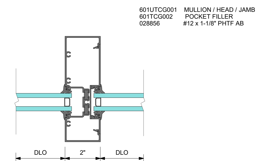
5 DETAIL 5 VERTICAL MULLION
