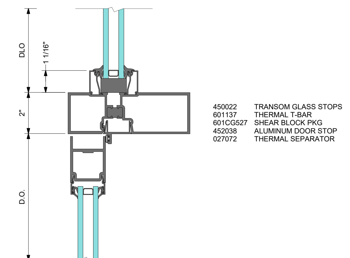
2 DETAIL 2 TRANSOM BAR WITH SURFACE CLOSER
