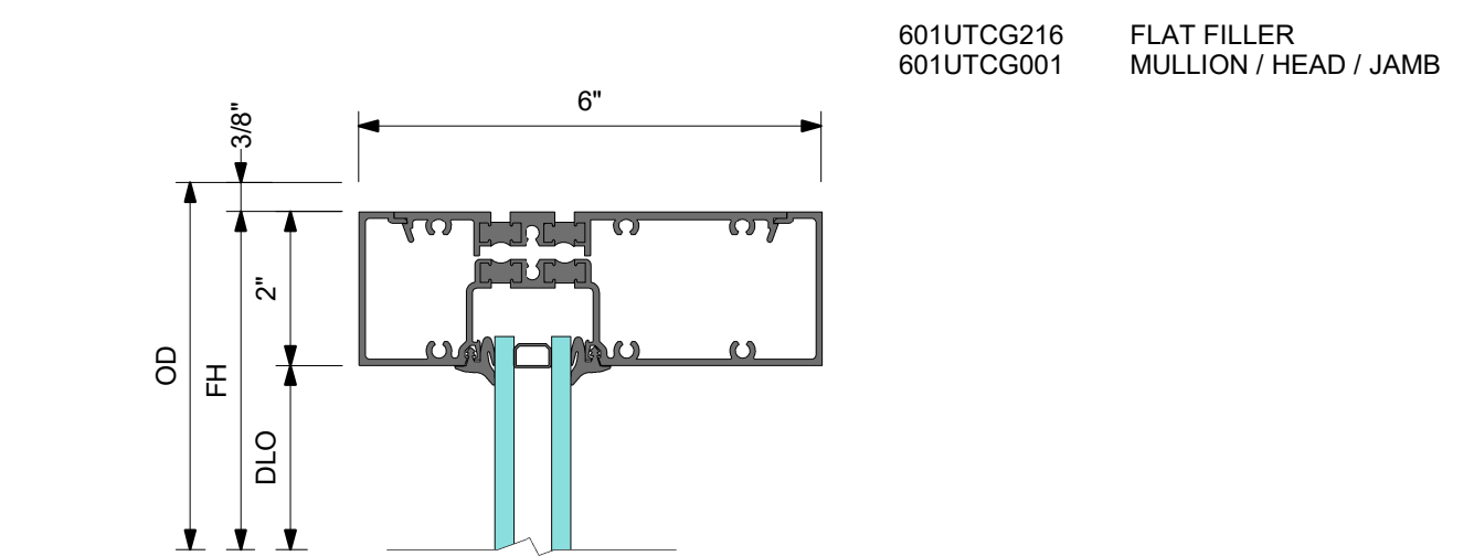
1 DETAIL 1 TRANSOM HEAD
