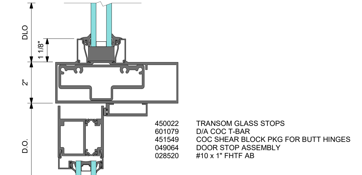
DOOR TRANSOM BAR WITH LCN CONCEALED CLOSER AND BUTT HINGES
