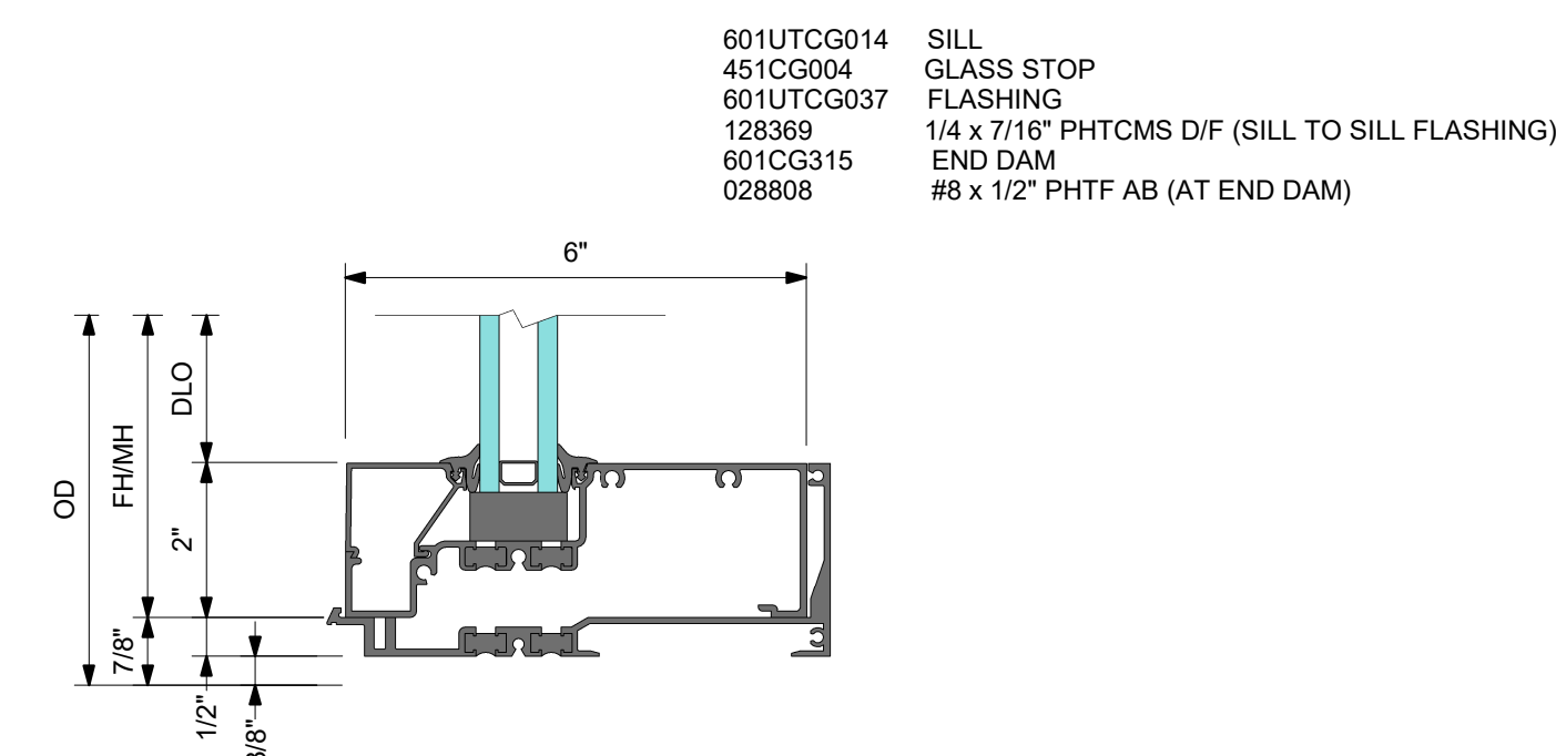
3 DETAIL 3 SILL
