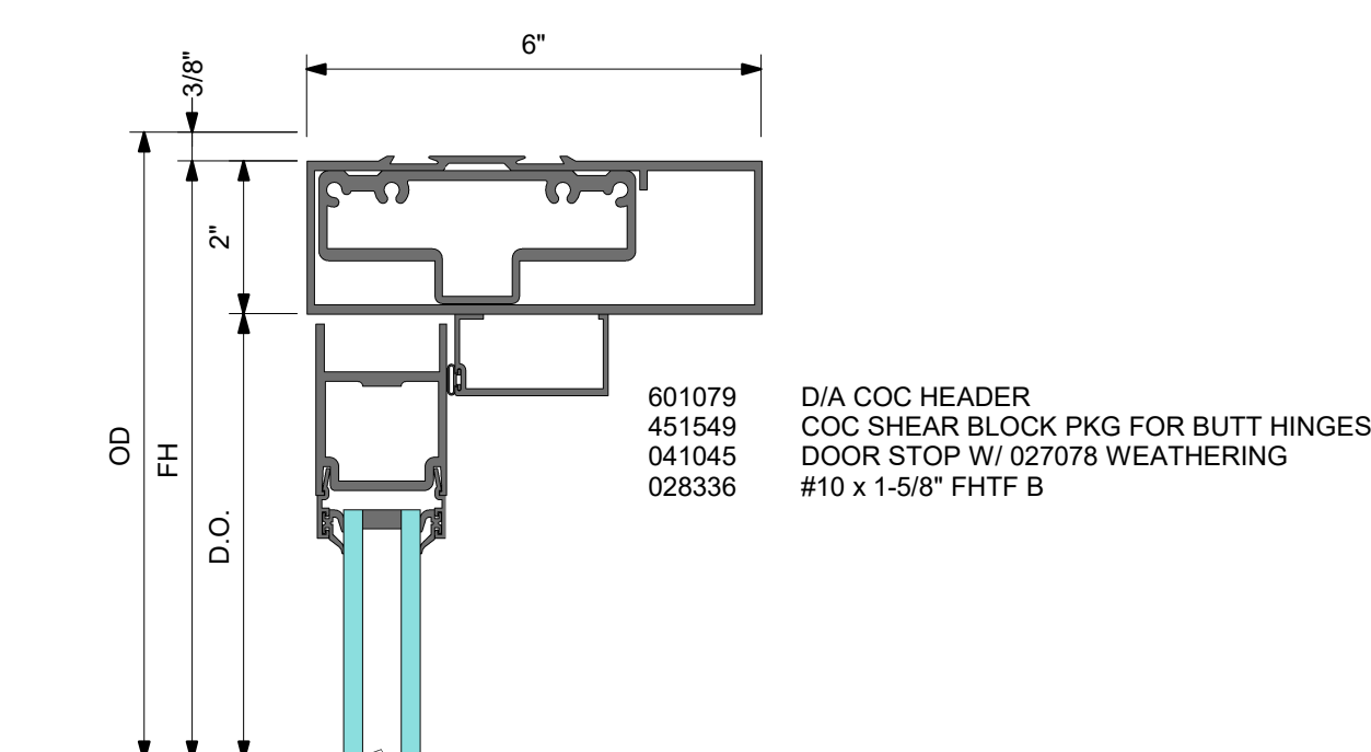
DOOR HEADER WITH KAWNEER CONCEALED CLOSER AND BUTT HINGES
