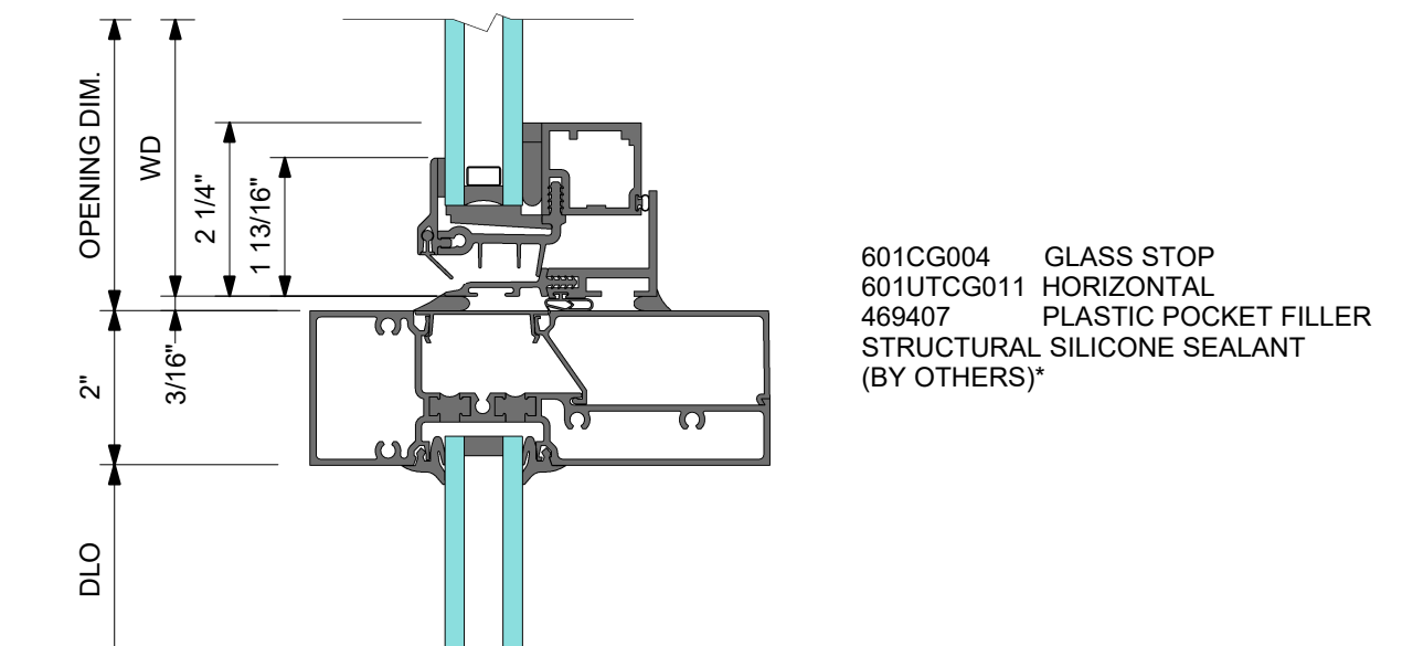
2 VENT SILL
