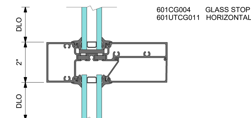
2 DETAIL 2 HORIZONTAL
