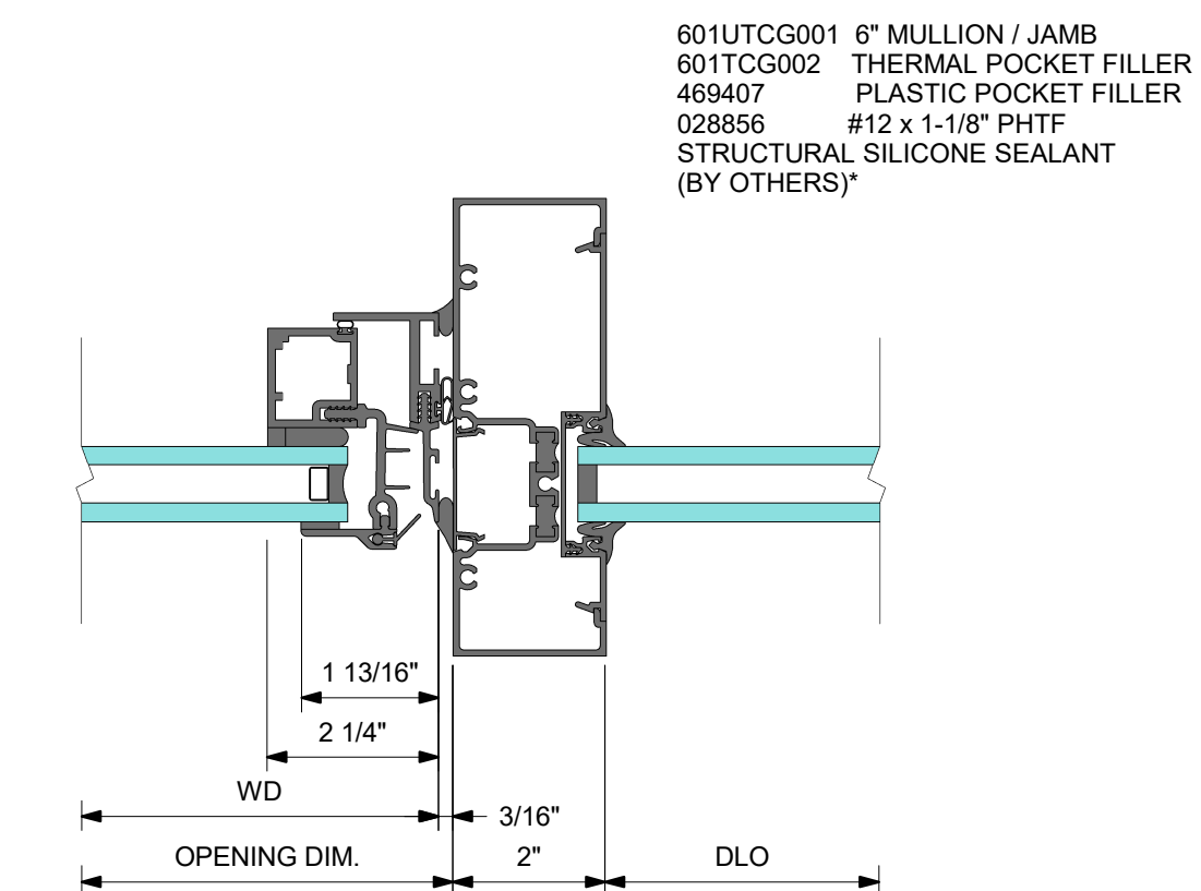
4 VENT @ LEFT
