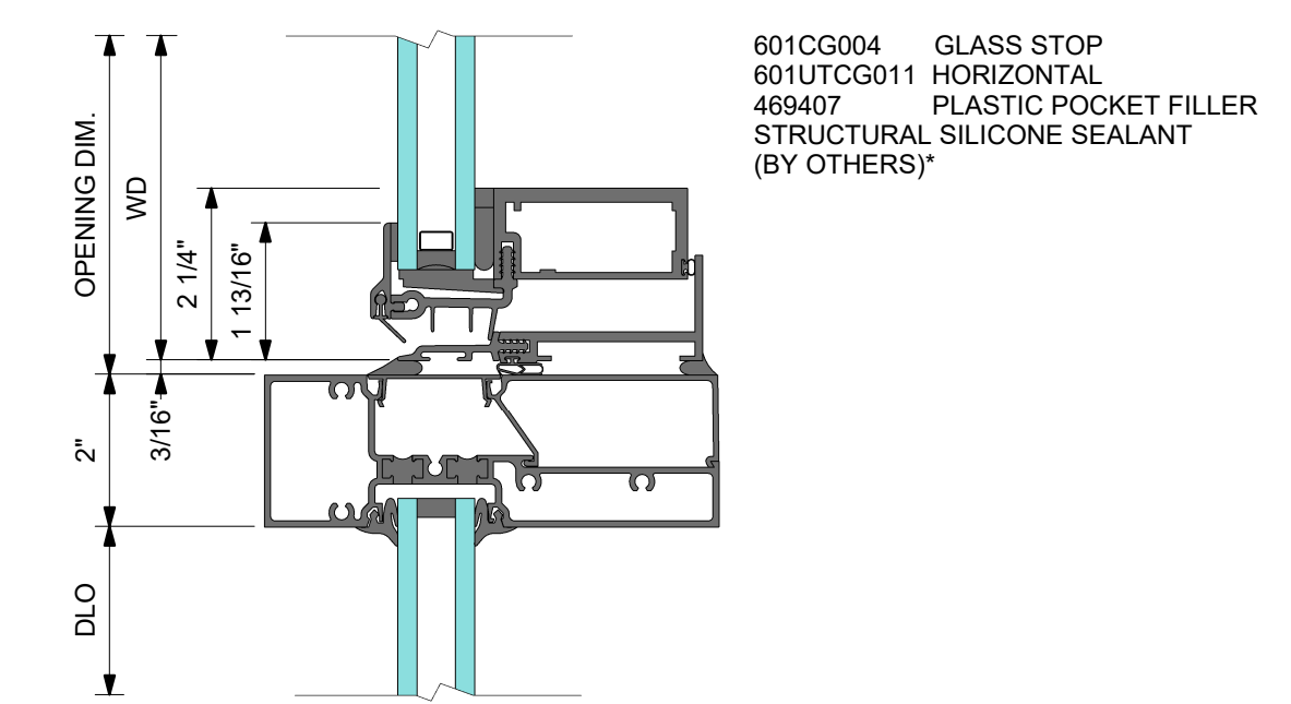
2 VENT SILL
