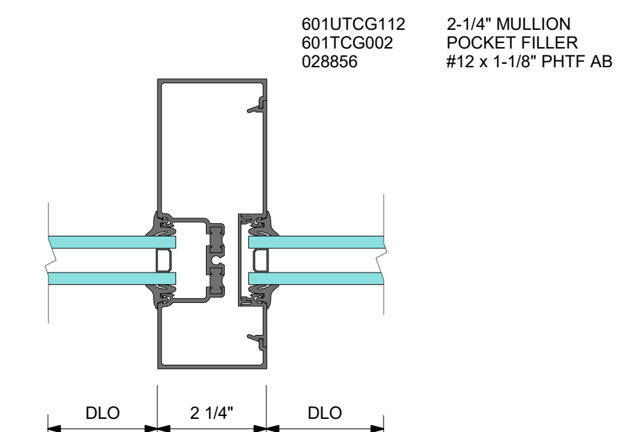
6 DETAIL 6 - 2-1/4" VERTICAL MULLION
